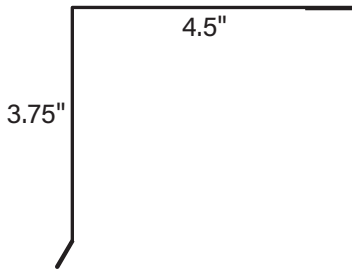
Gable Trim
