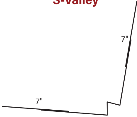
S-Valley
